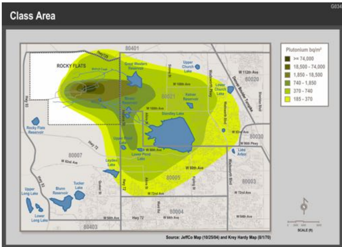
Figure 2: The enhanced version of the Krey Hardy map with colored plutonium isopleths in Bq/m 2 . Note that 1,850 Bq/m 2 represents 171x background radiation, using 0.0434 dpm/g as background.
